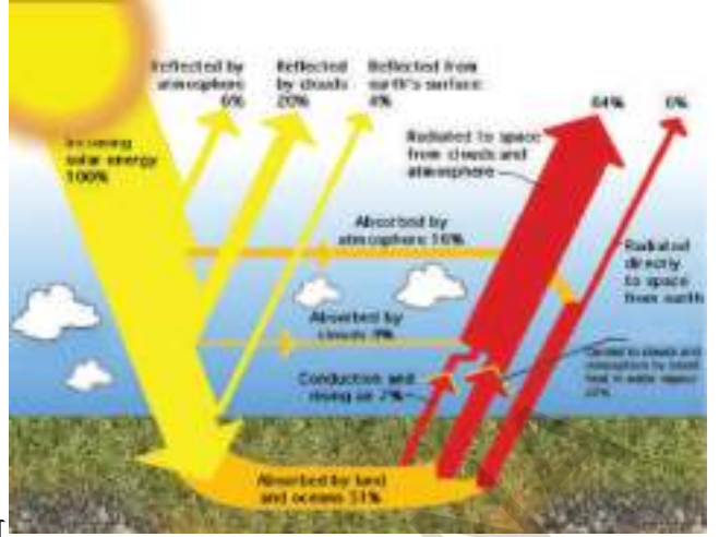
चित्र 2.2: Insolation and terrestrial radiation
